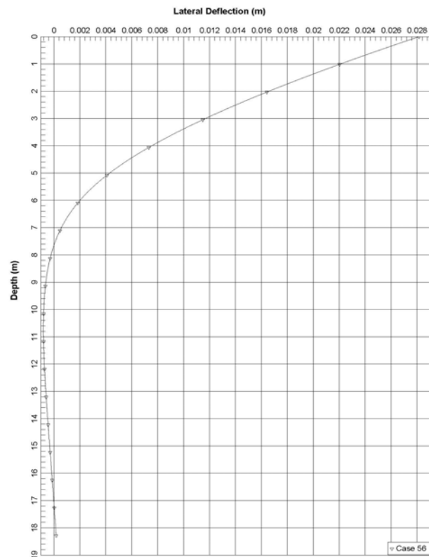
Figure 4b Lateral movement based on PMT-PY curves
