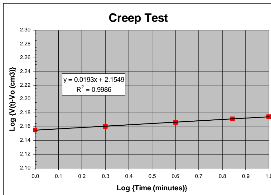
Figure 2. Creep test results from above PMT
