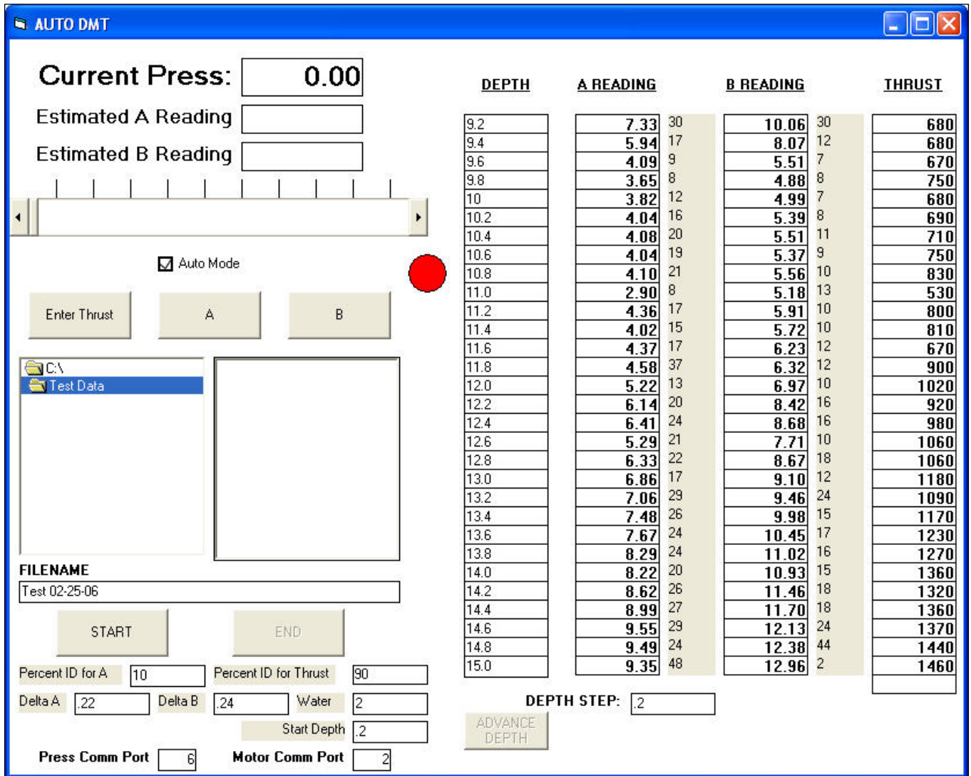
Figure 2: Screen shot of AutoDMT program
